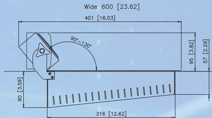
SUNK INTO CUSTOM WOODWORK Dimensions in mm [inches]
